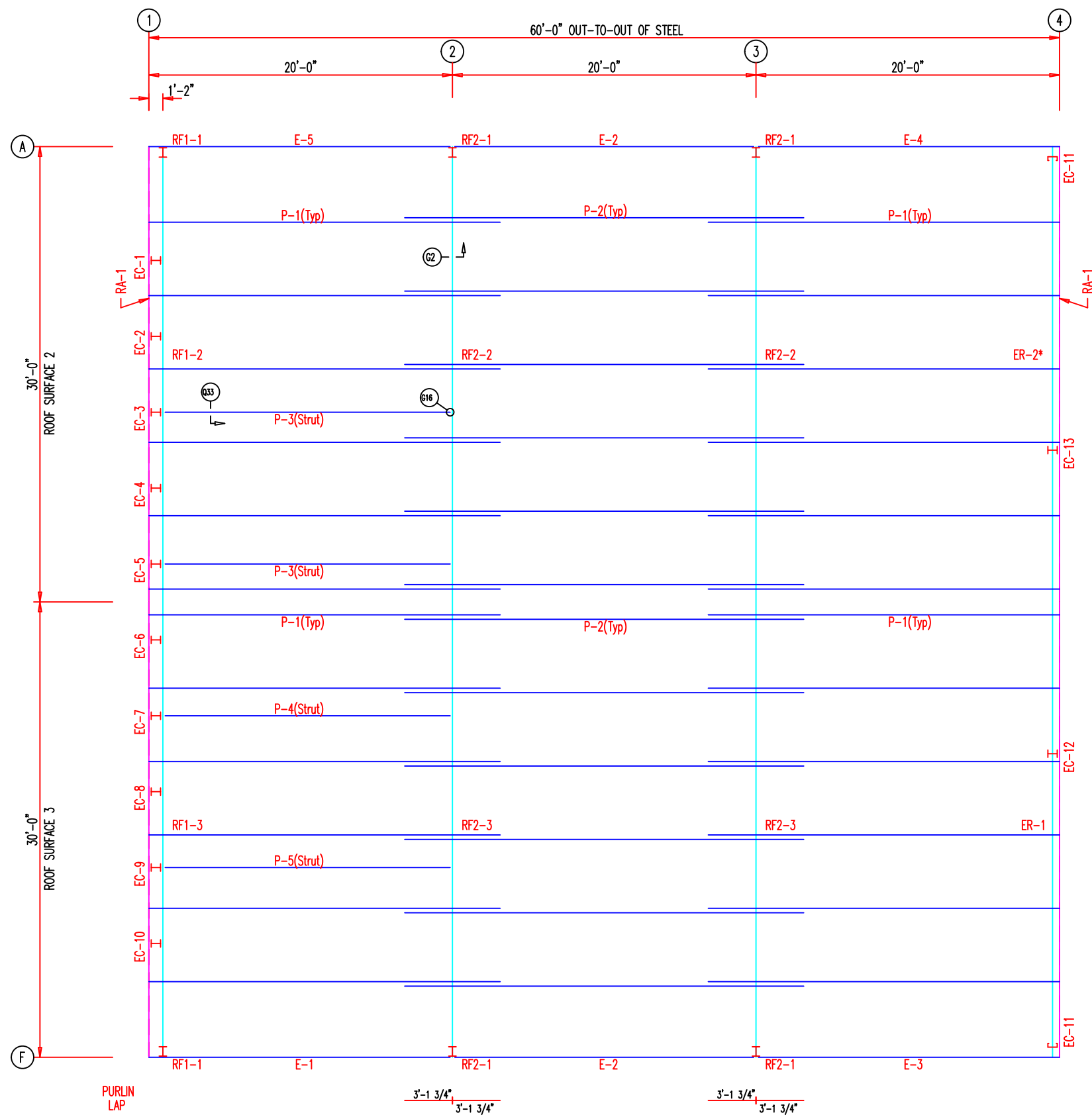
ROOF FRAMING PLAN
