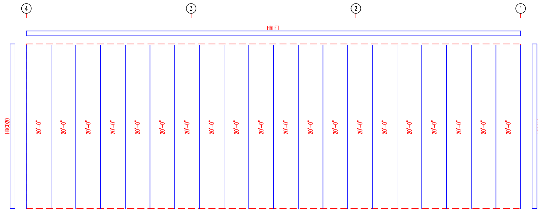
SIDEWALL SHEETING & TRIM: FRAME LINE A
